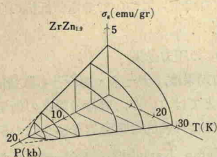
Fig. 13 Magnetization per gram of ZrZn_{19} as a function of temperature and pressure, which is made from the data of Ref. 80.
